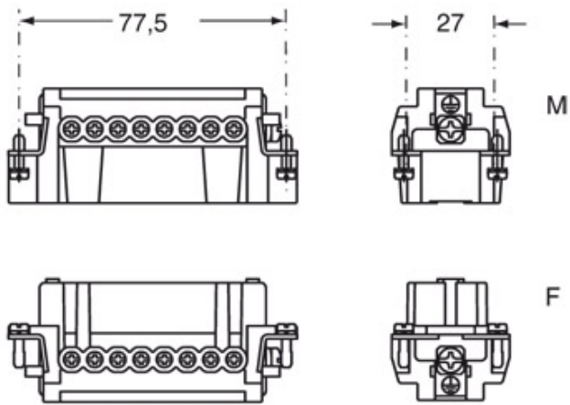
Catalogue drawings
