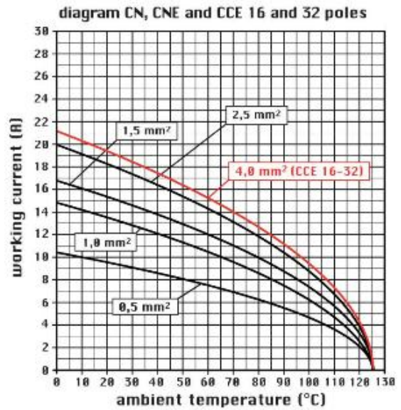
Catalogue drawings
